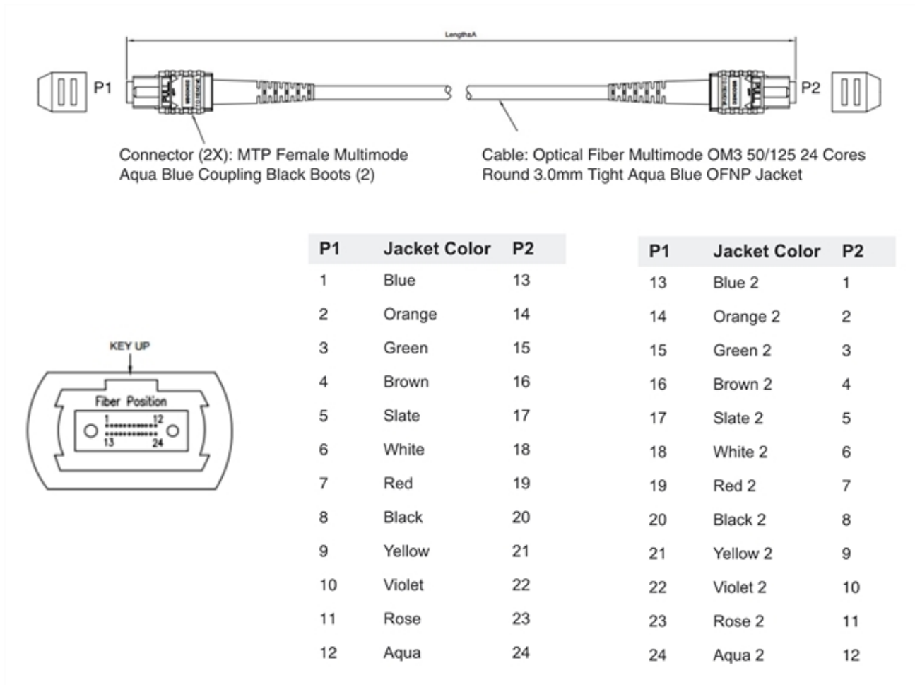
Figure 20 MPO/MTP 24 Position Fiber Cable
