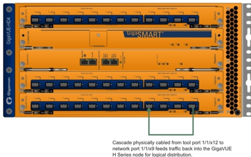
Figure 160 Cascade Physically Cabled from Tool to Network Port
