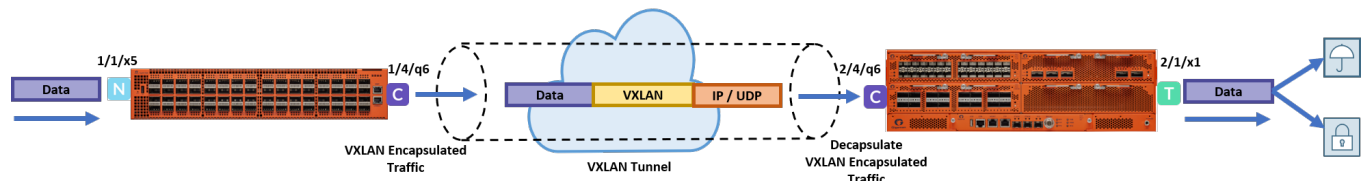
Figure 30 VXLAN Tunnel Encapsulation and Decapsulation
