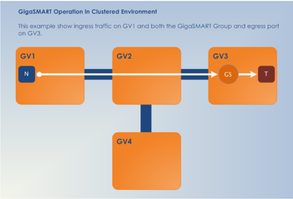
Figure 153 GigaSMART Operations in Clusters
