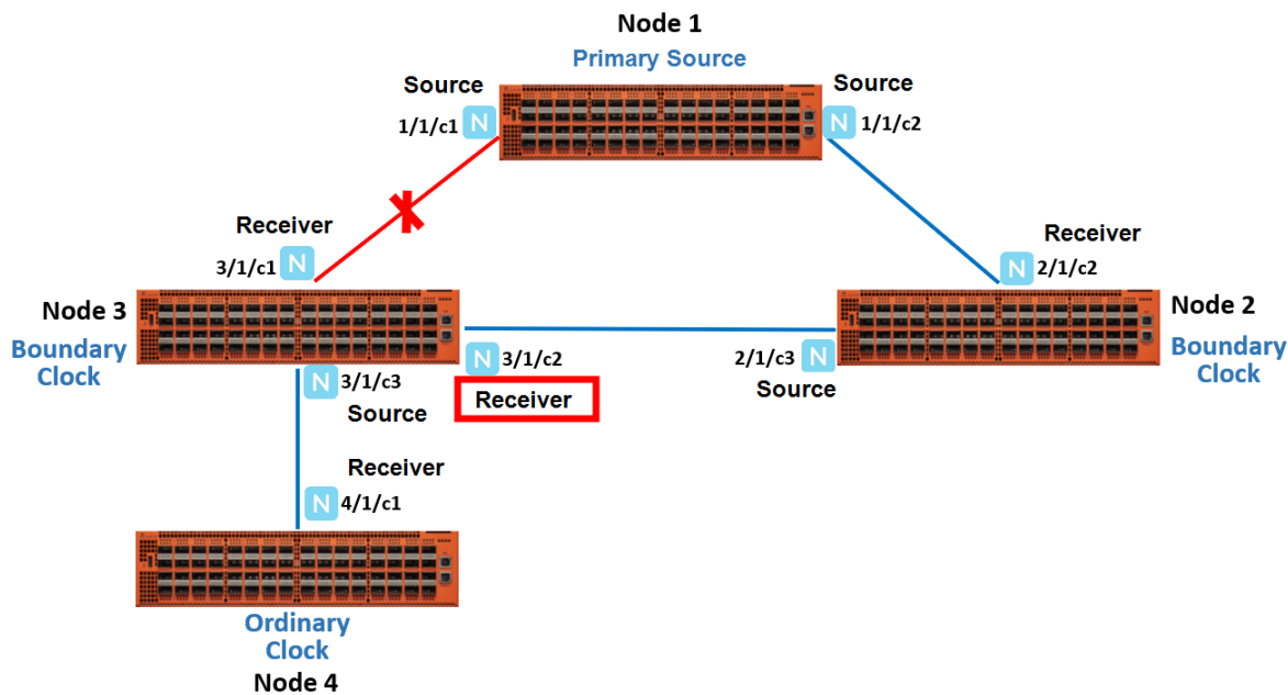
Figure 20 PTP State Transition
