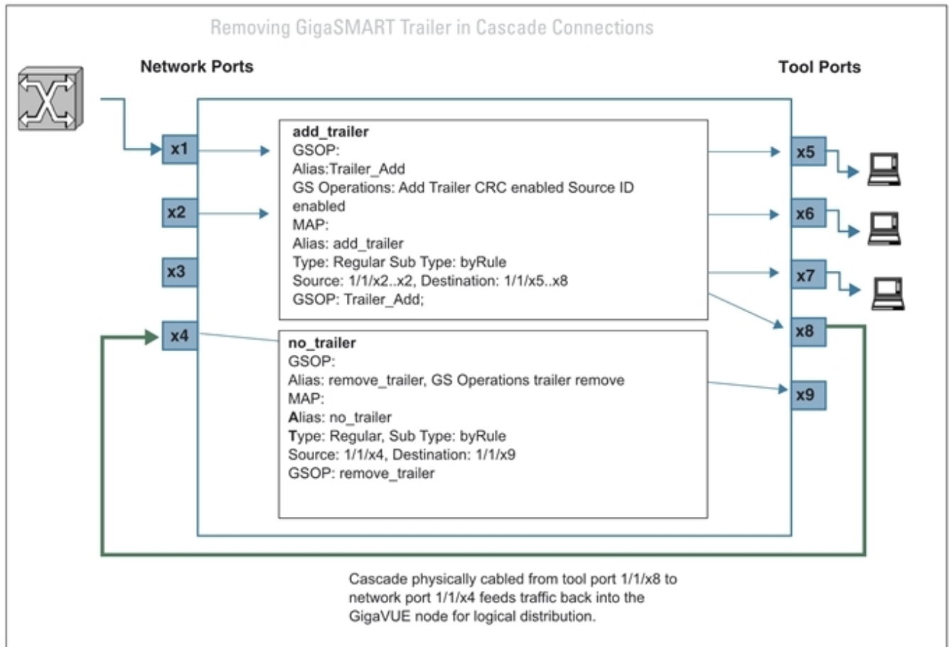
Figure 161 Removing the GigaSMART Trailer from a Cascade Connection
