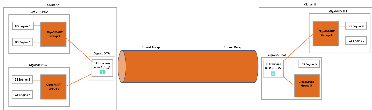
Figure 134 Tunnel Centralization
