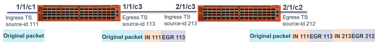
Figure 18 Timestamping
