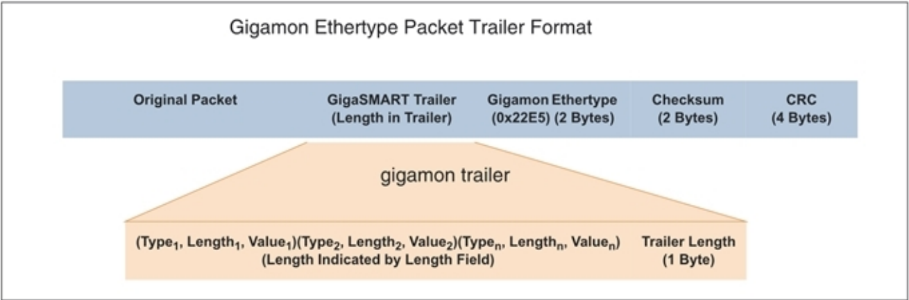
Figure 162 GigaSMART Trailer Format
