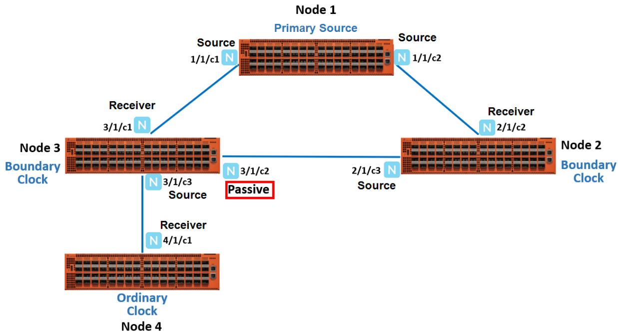
Figure 19 PTP Deployment
