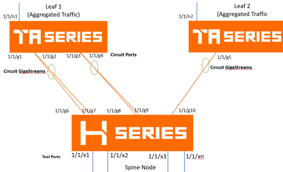
Figure 26 Circuit GigaStreams in Fabric Maps
