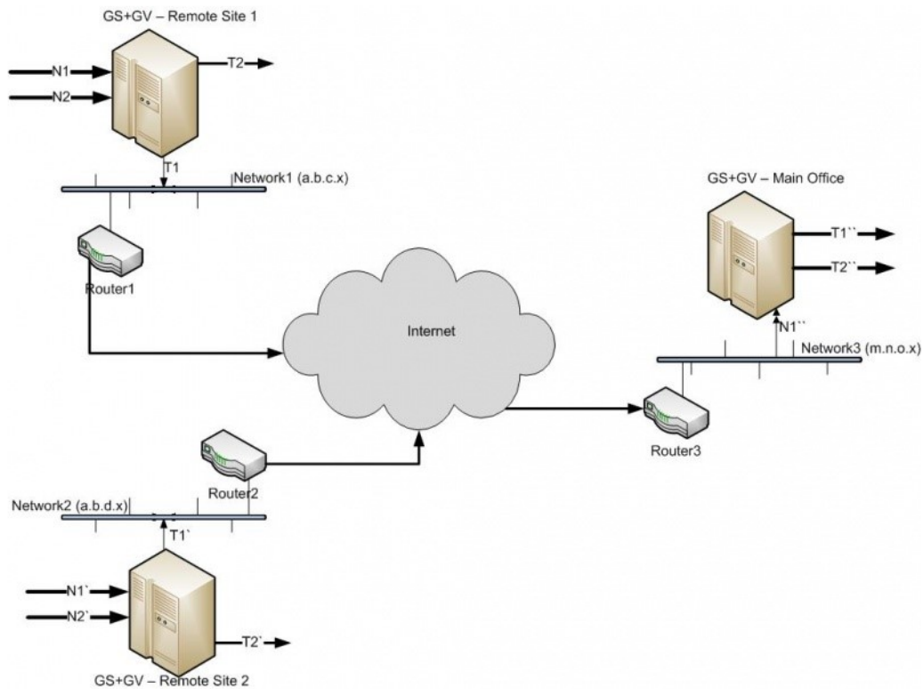
Figure 135 L2GRE Tunnel Encapsulation/Decapsulation
