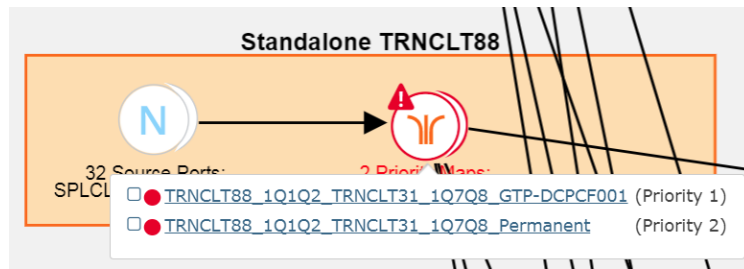
Figure 17 Unhealthy Maps
