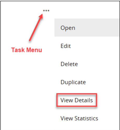
Figure 66 View Details.
