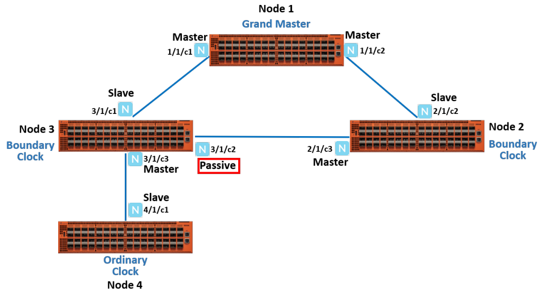
Figure 58 PTP Deployment
