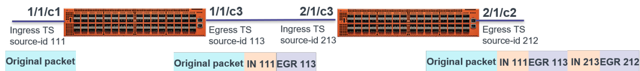
Figure 57 Timestamping
