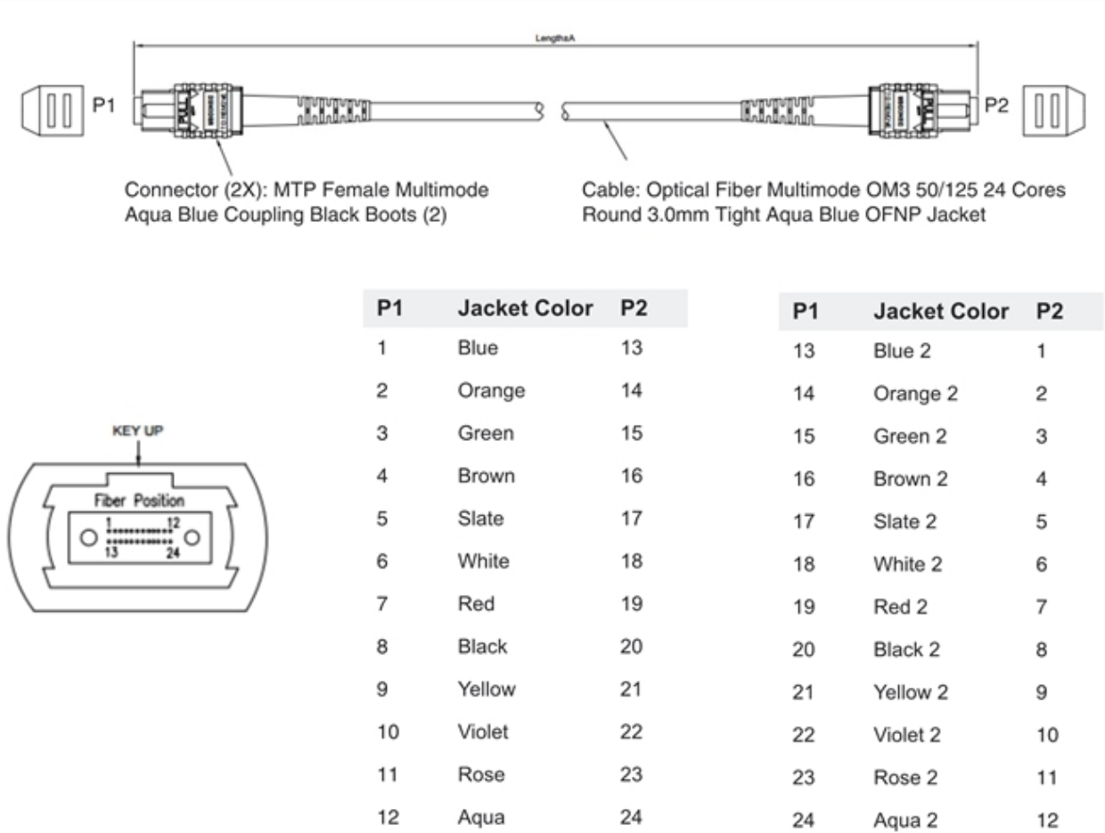
Figure 22 MPO/MTP 24 Position Fiber Cable
