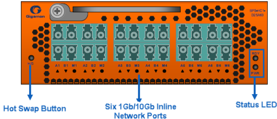
Figure 4 BPS-HC1-D35C60
