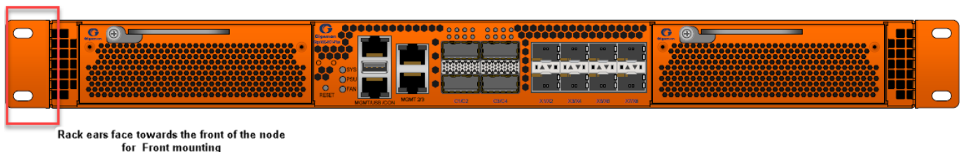
Front Mount GigaVUE-HC1P
