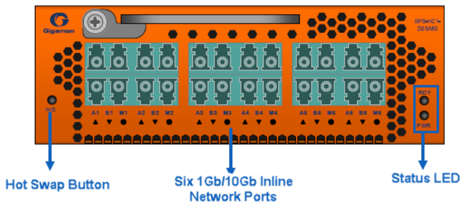
Figure 5 Bypass Combo Module BPS-HC1-D25A60
