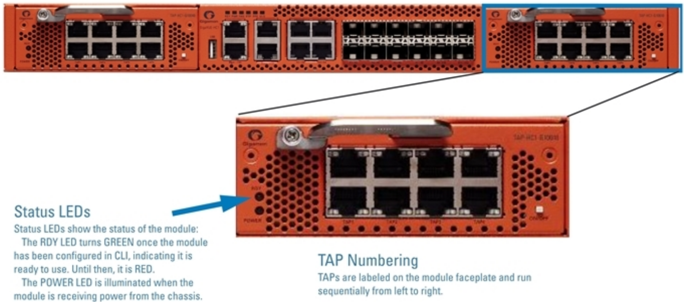
Figure 8 TAP-HC0-G10040 Module
