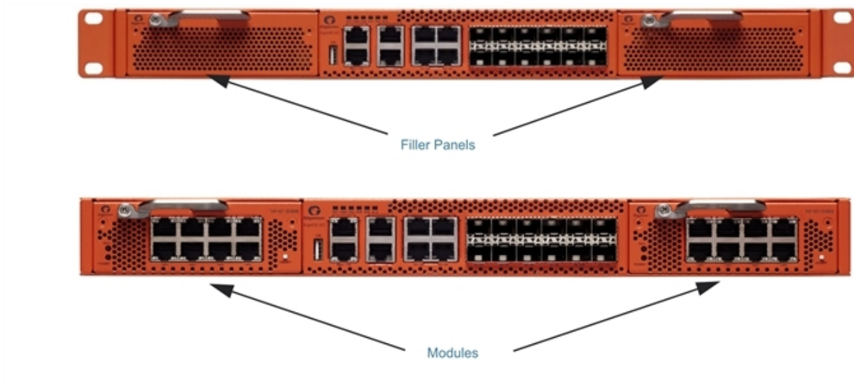
Figure 4 Installing Modules
