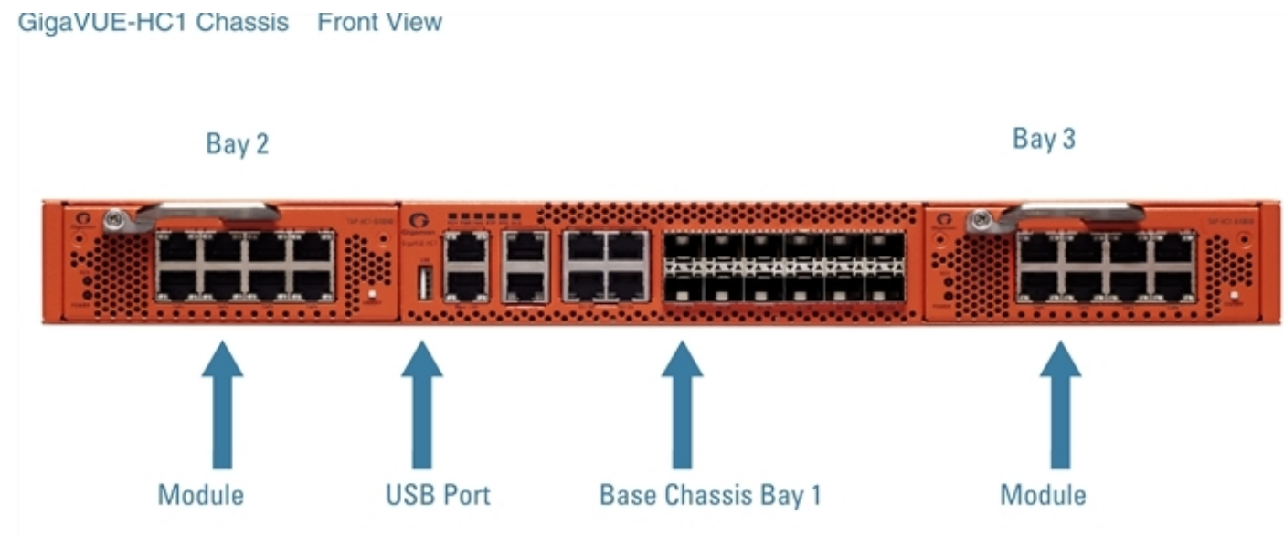
Figure 1 Front View of the GigaVUE-HC1 Chassis
