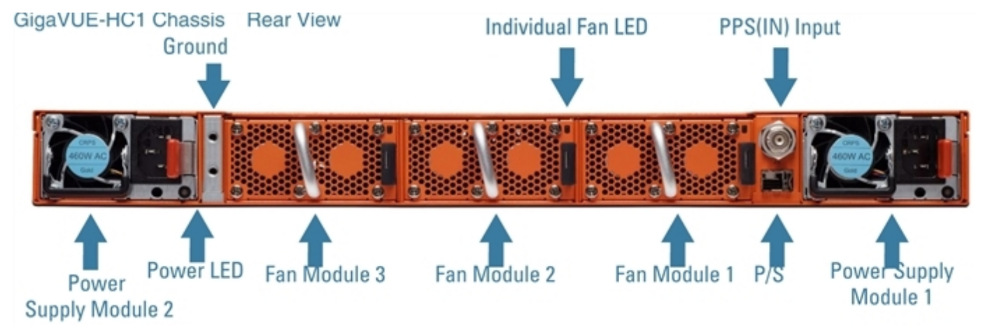
Figure 2 Rear View of the GigaVUE-HC1 Chassis
