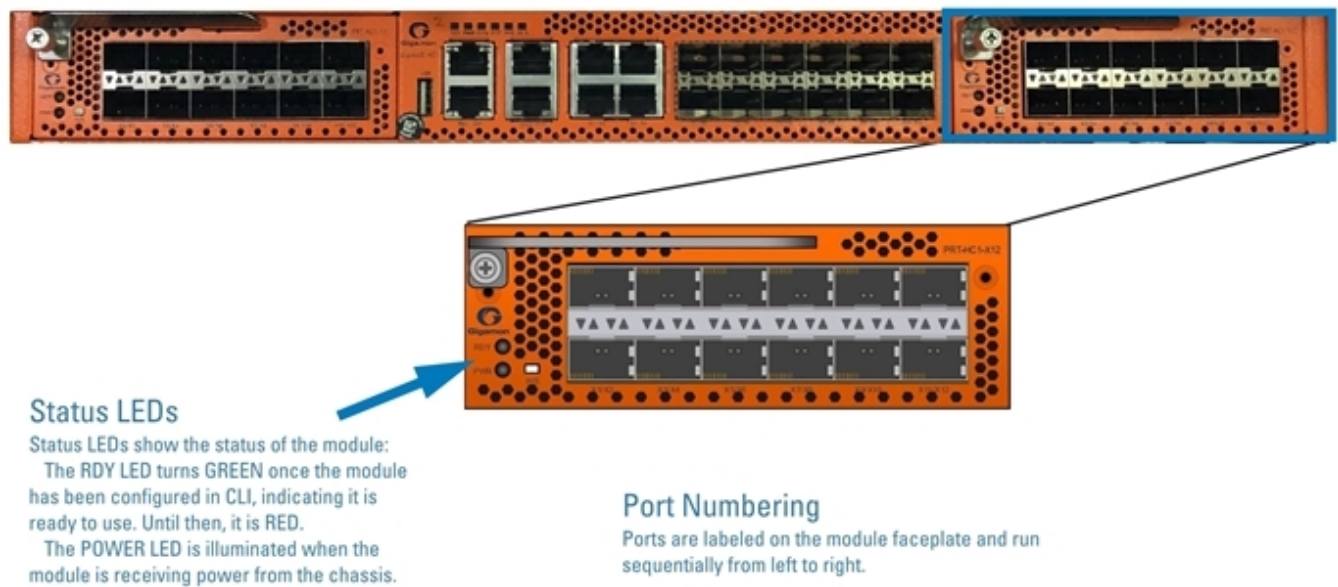
Figure 7 PRT-HC1-X12 Module
