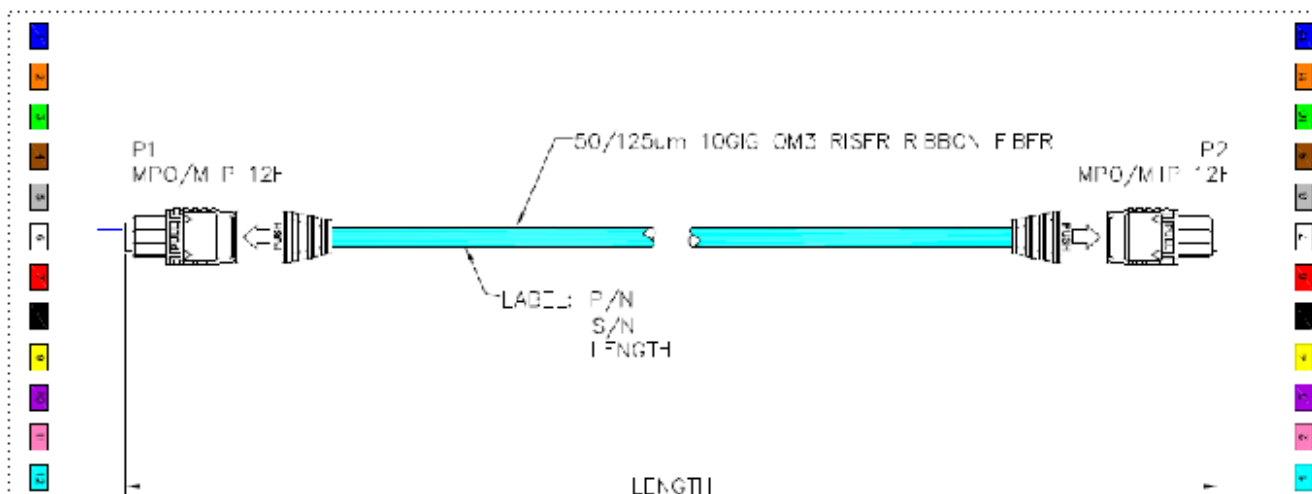
Figure 17 MPO/MTP 12 Position Fiber Cable
