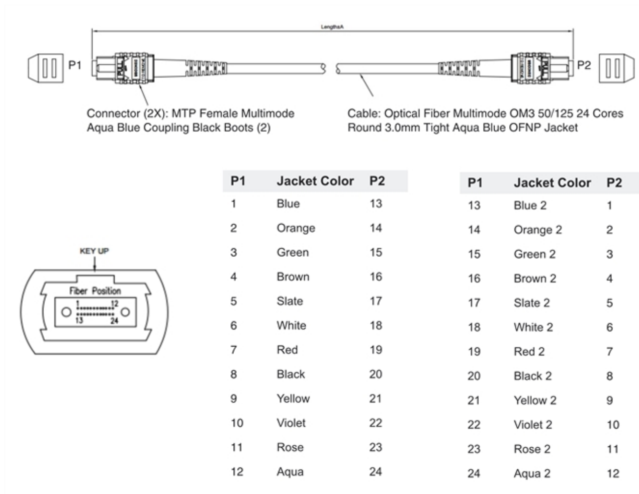
Figure 19 MPO/MTP 24 Position Fiber Cable
