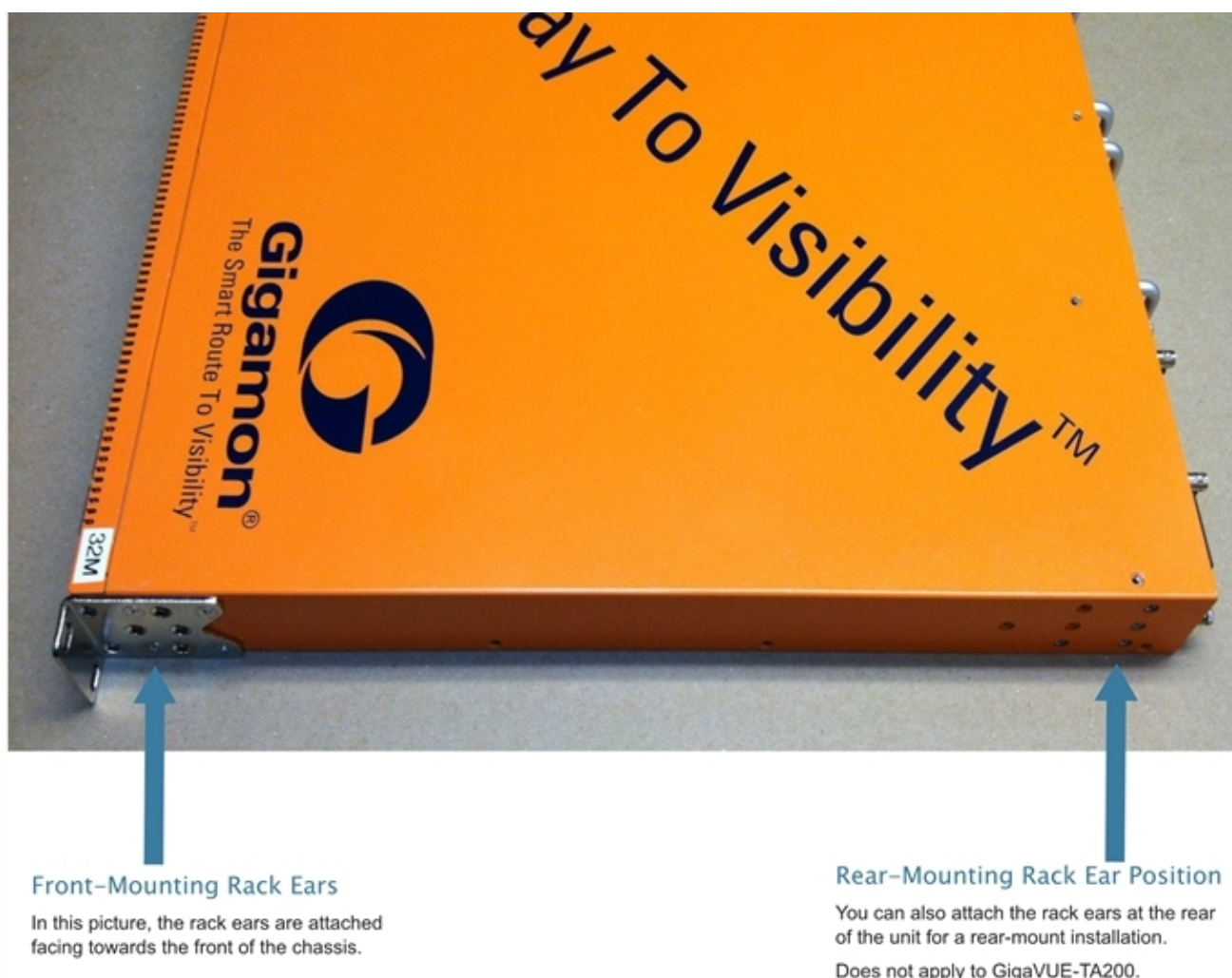
Figure 1 GigaVUE TA Series Traffic Aggregator Rack Ears in Front-Mount Position
