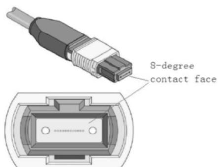
Figure 18 MTP/APC Cable
