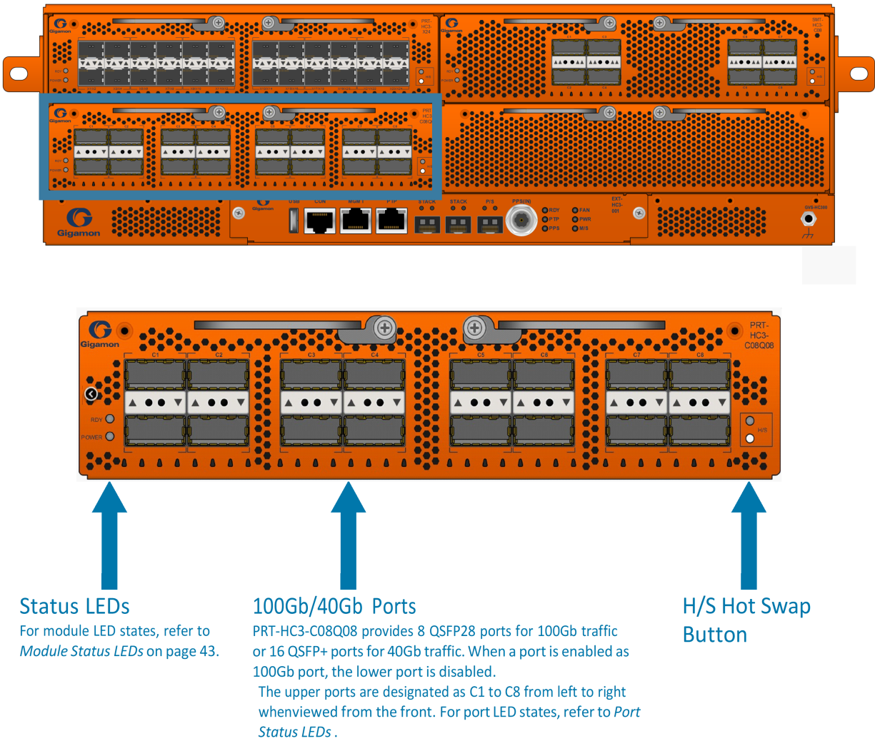
Figure 5 PRT-HC3-C08Q08 Module
