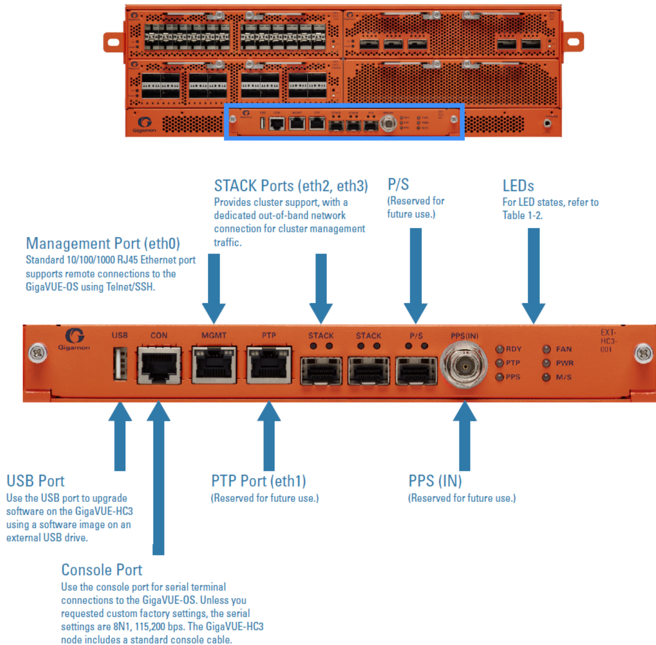
Figure 3 GigaVUE-HC3 Extension Board
