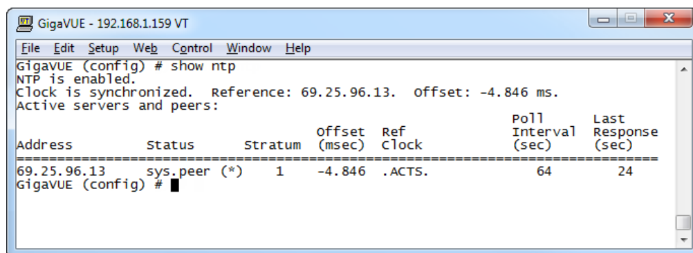
Figure 26 Checking NTP Status and Configuration
