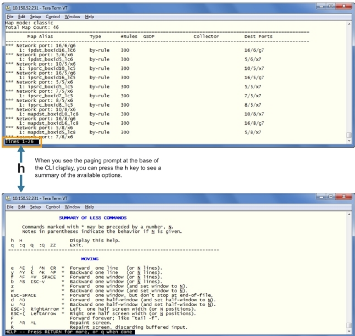
Figure 25 Viewing Paging Options
