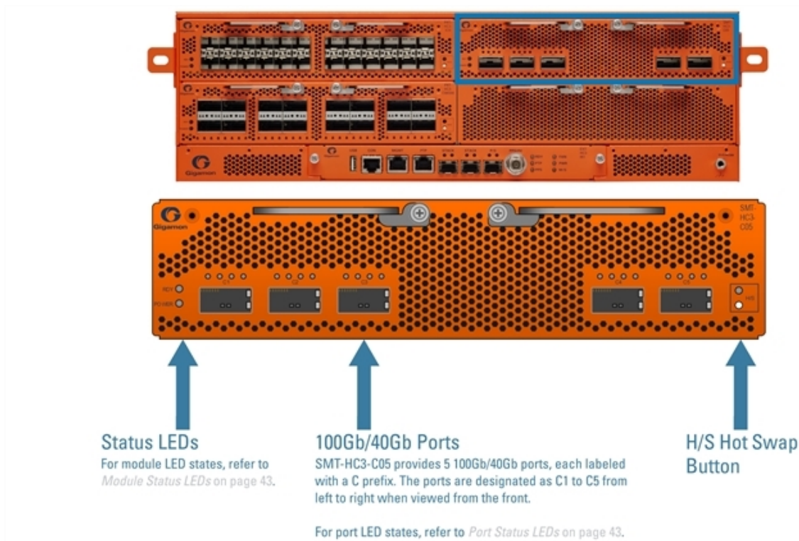
Figure 7 SMT-HC3-C05 Module
