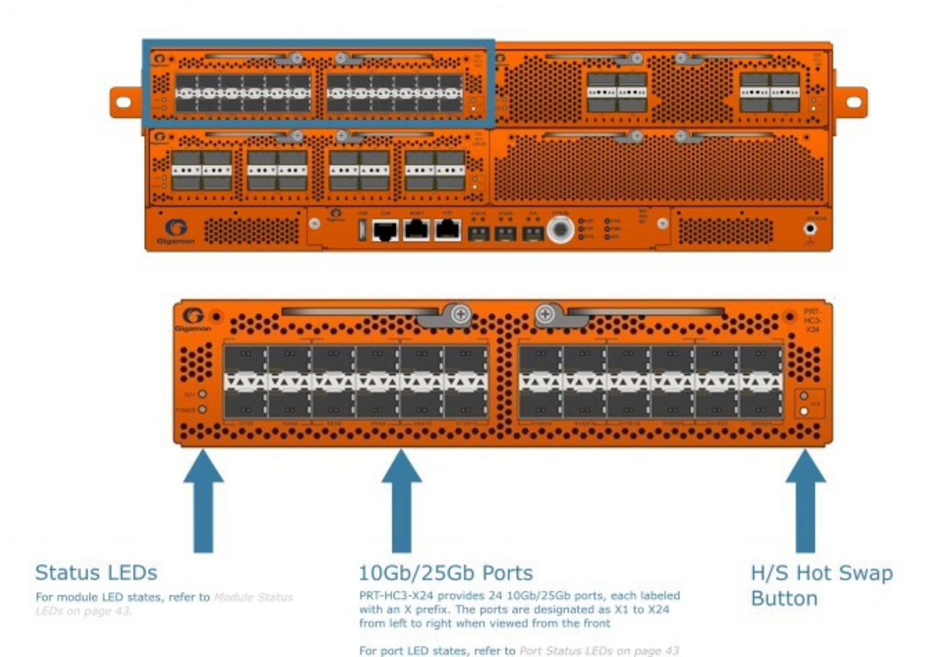
Figure 4 PRT-HC3-X24 Module
