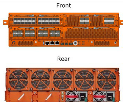
GigaVUE-HC3
