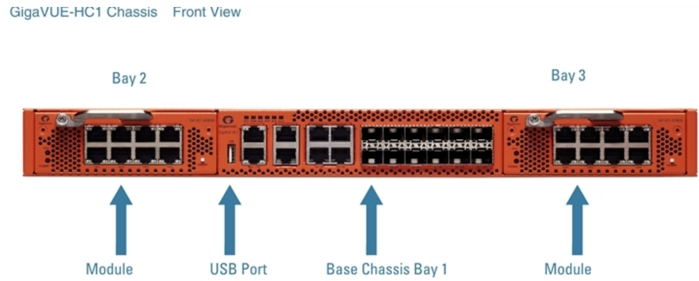
Figure 1 Front View of the GigaVUE-HC1 Chassis
